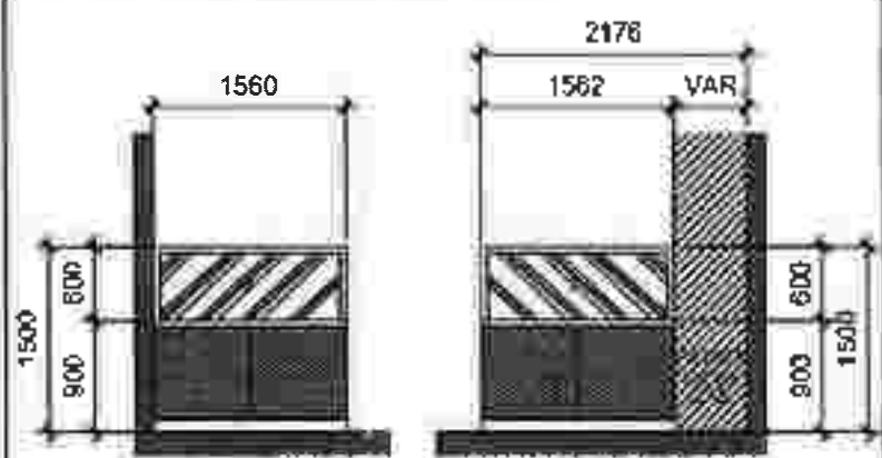
ELEV. A ELEV. B LOW PARTITION ELEVATION
