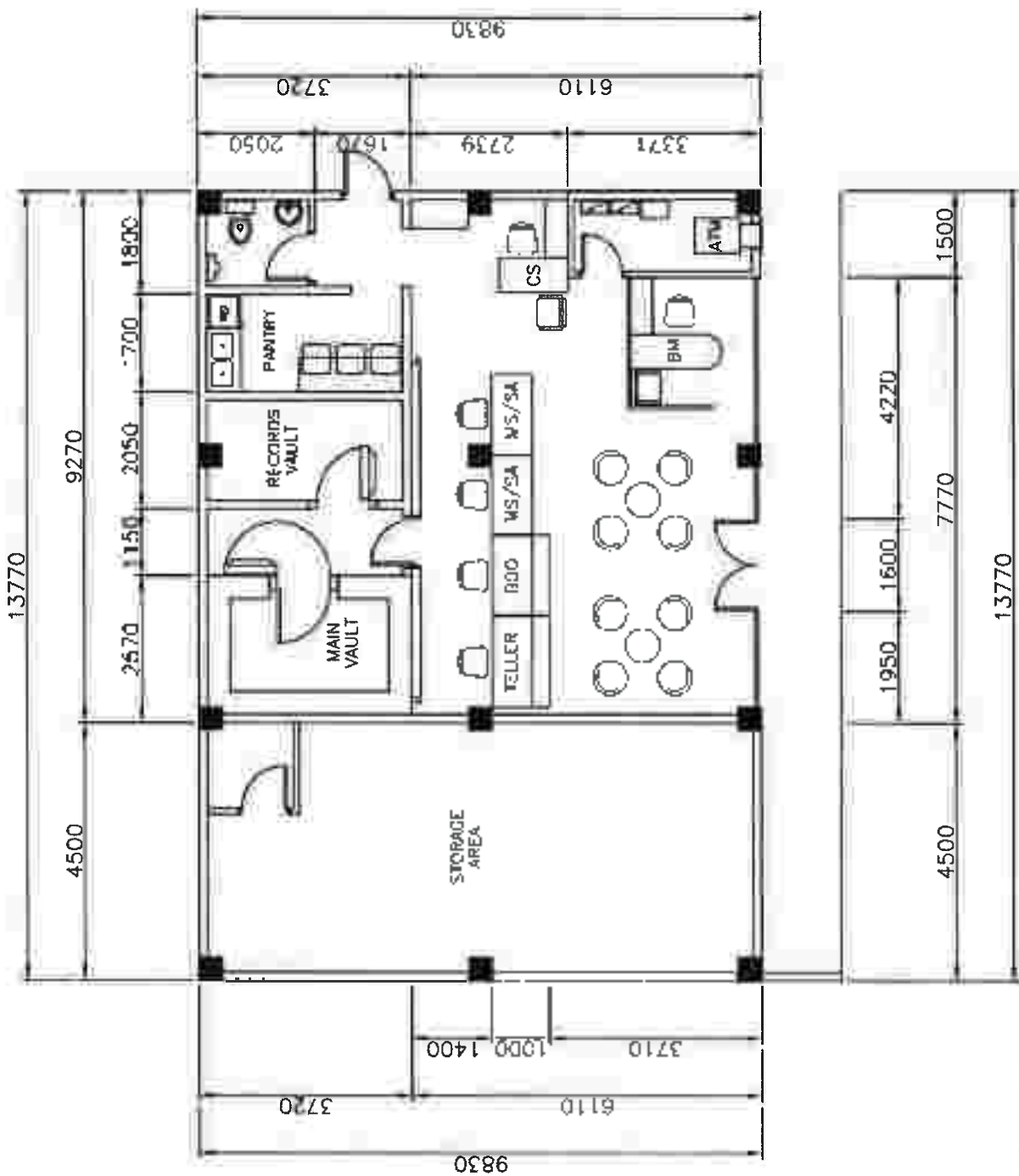
EXISTING UCPBS BACNOTAN BRANCH FLOOR LAY-OUT
