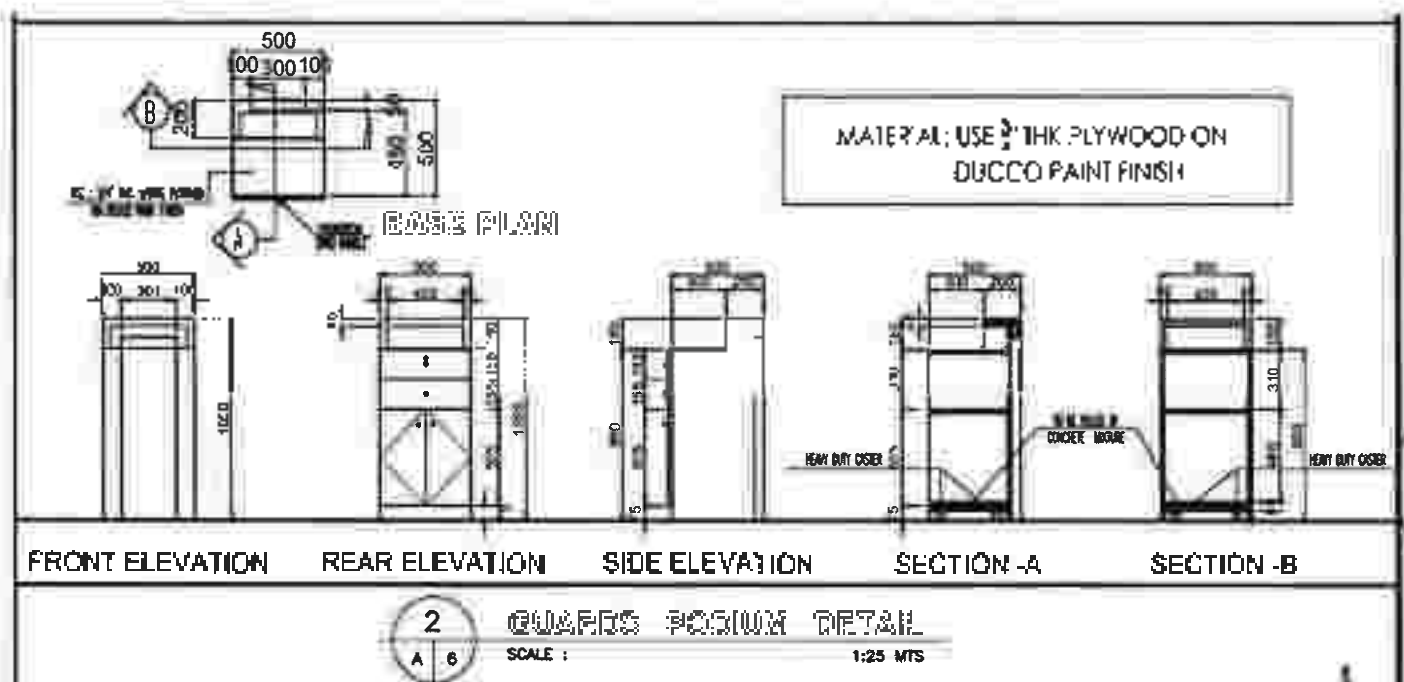
GUARDS PODIUM DETAILS
